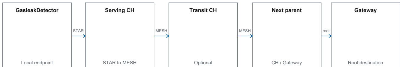
Figure 1. Serving and transit roles in the field path.
