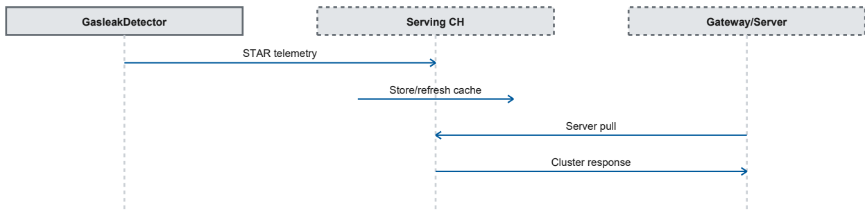
Figure 7. Cache/pull path for normal telemetry.
